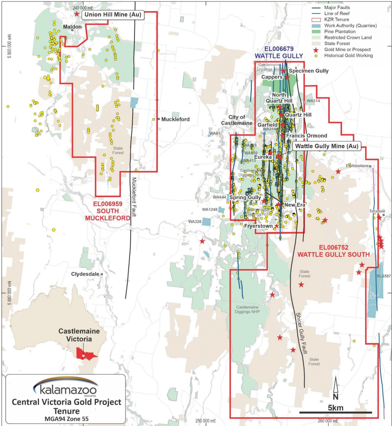
Figure 1: South Muckleford EL6959 location
